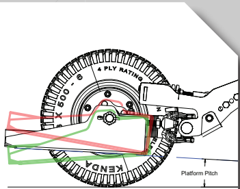
ADJUSTABLE PLATFORM PITCH (ALL MODELS)
