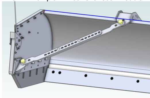
8-12' Example Arm Stiffener Use—Double
